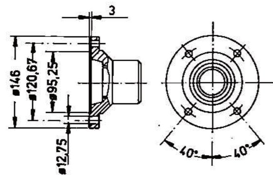
BRIDA 1500 SAE
